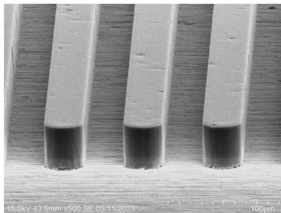
HT215F 22/41sst L/S=34 µm/34 µm
