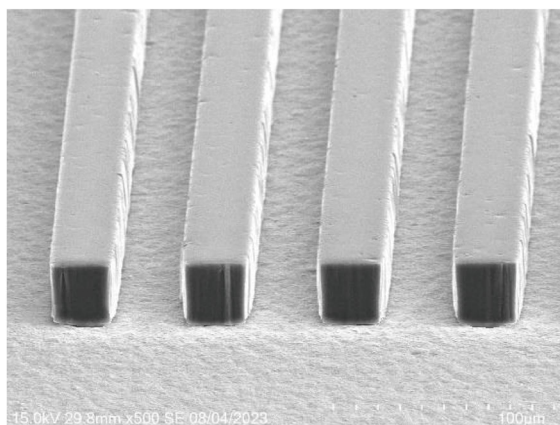
HT2612 19/41sst L/S=30 µm/30 µm
